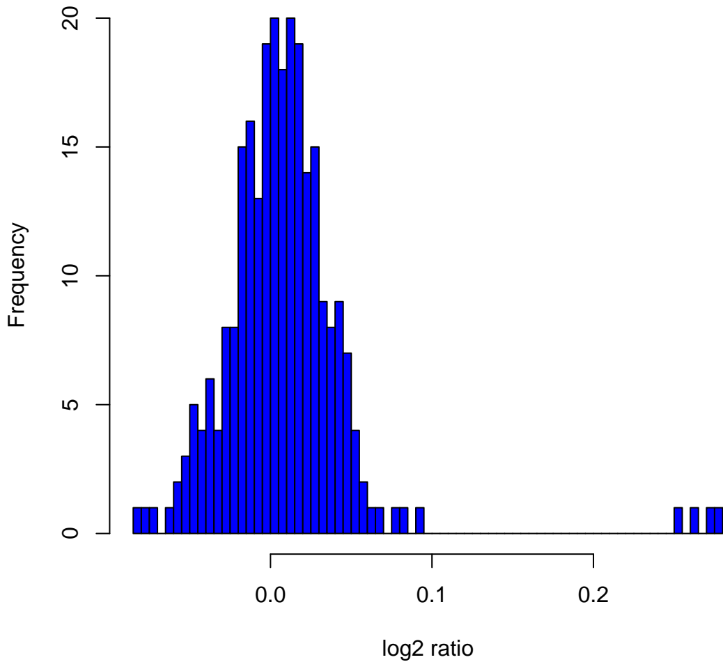
Histogram of log 2 ratios in 270 HapMap samples at clone Chr7tp-5H5
