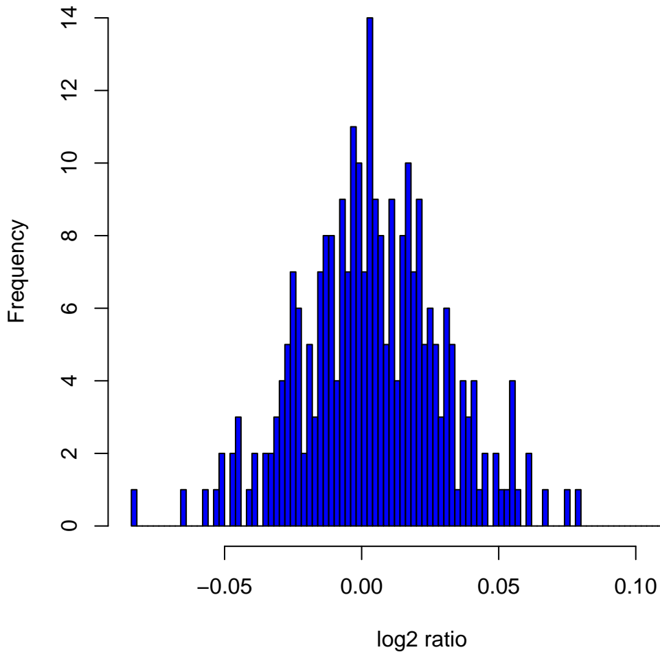
Histogram of log 2 ratios in 270 HapMap samples at clone Chr7tp-7B11
