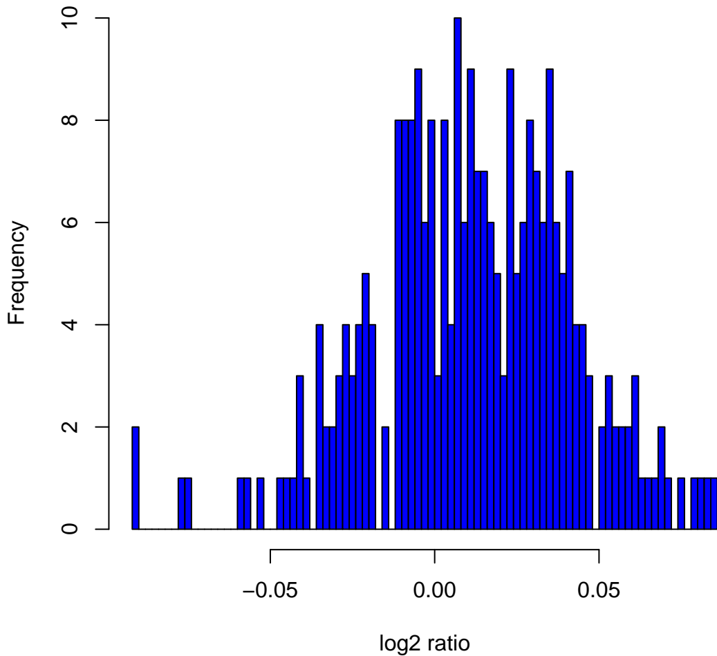
Histogram of \log_2 ratios in 270 HapMap samples at clone Chr7tp-7D9
