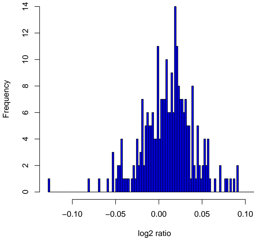
Histogram of log 2 ratios in 270 HapMap samples at clone Chr7tp-7E1
