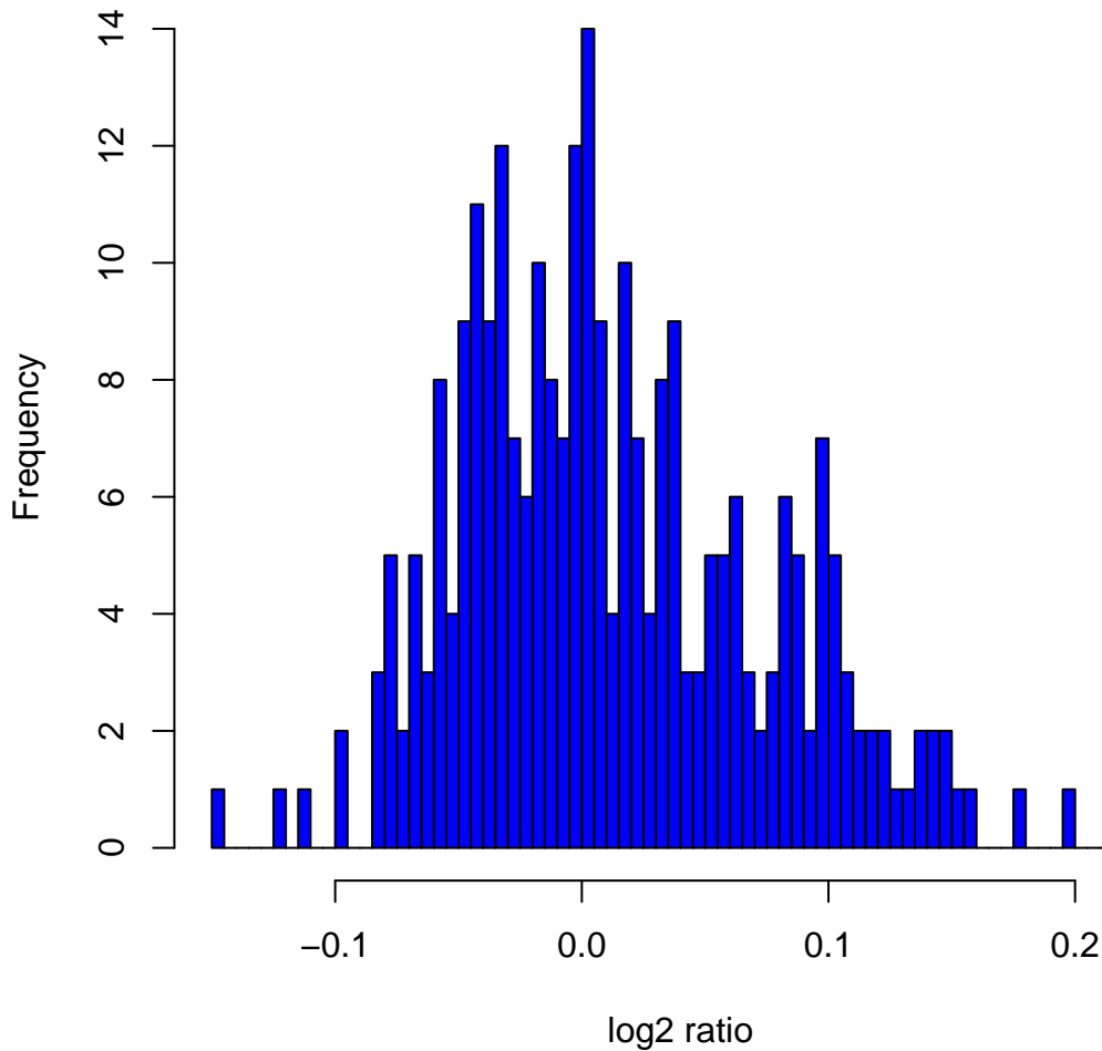
Histogram of \log_2 ratios in 270 HapMap samples at clone Chr7tp-7G10
