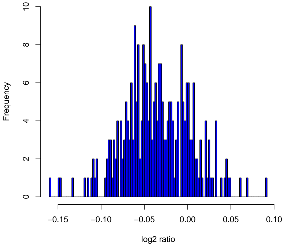
Histogram of log 2 ratios in 270 HapMap samples at clone Chr7tp-7G4
