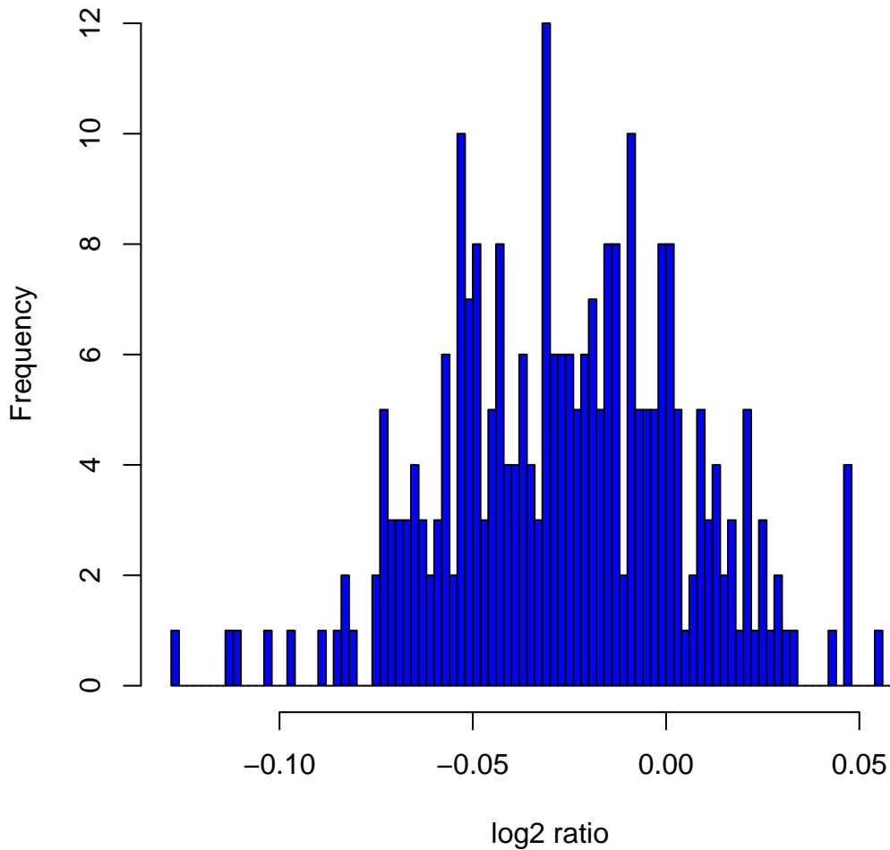
Histogram of log 2 ratios in 270 HapMap samples at clone Chr7tp-7H3
