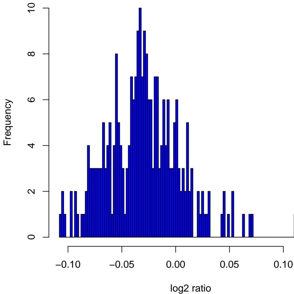
Histogram of \log_2 ratios in 270 HapMap samples at clone Chr7tp-8C10
