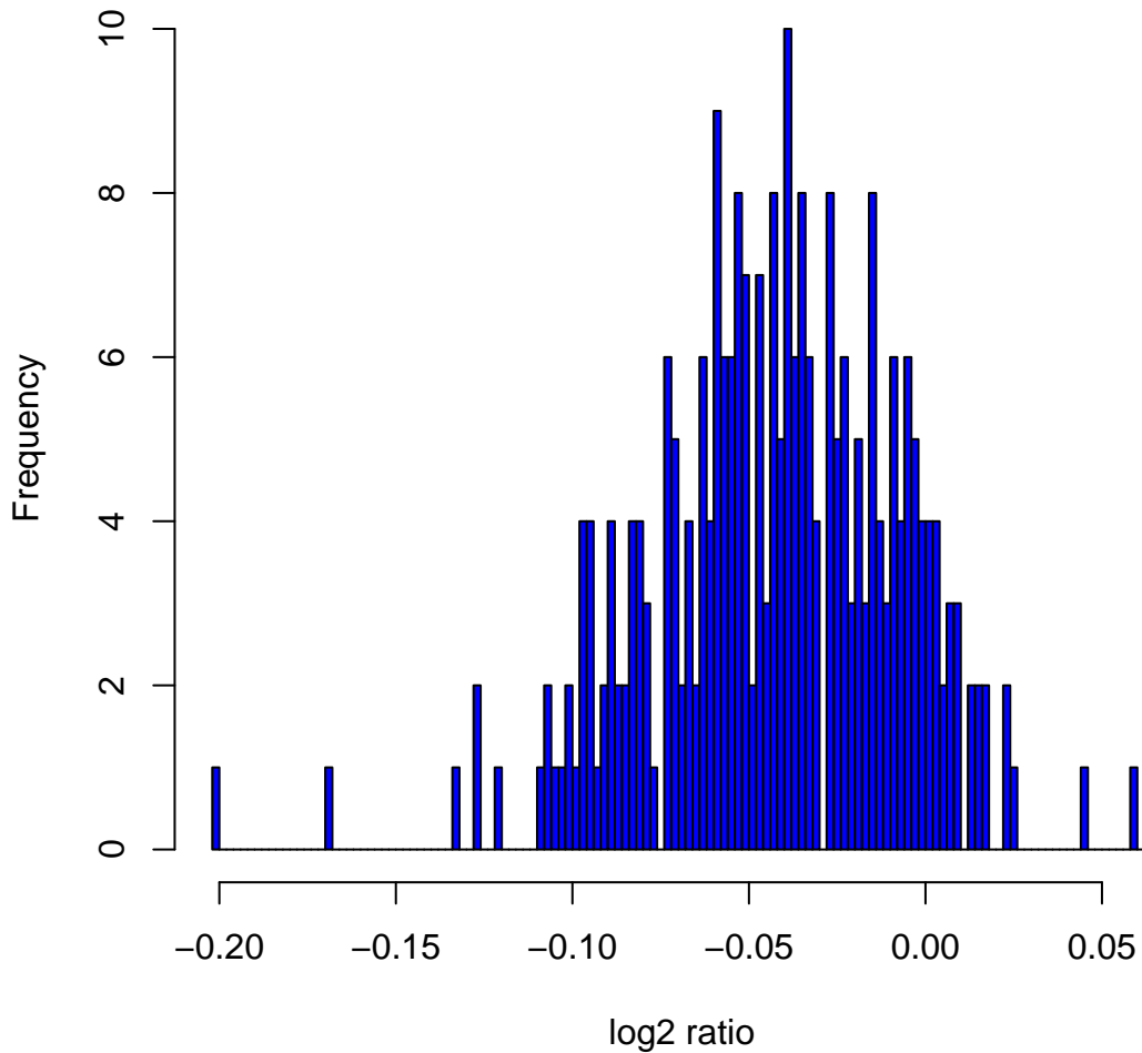
Histogram of log 2 ratios in 270 HapMap samples at clone Chr7tp-8D8
