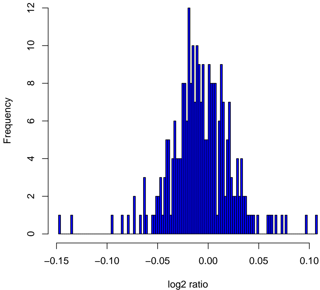
Histogram of log 2 ratios in 270 HapMap samples at clone Chr7tp-8G2
