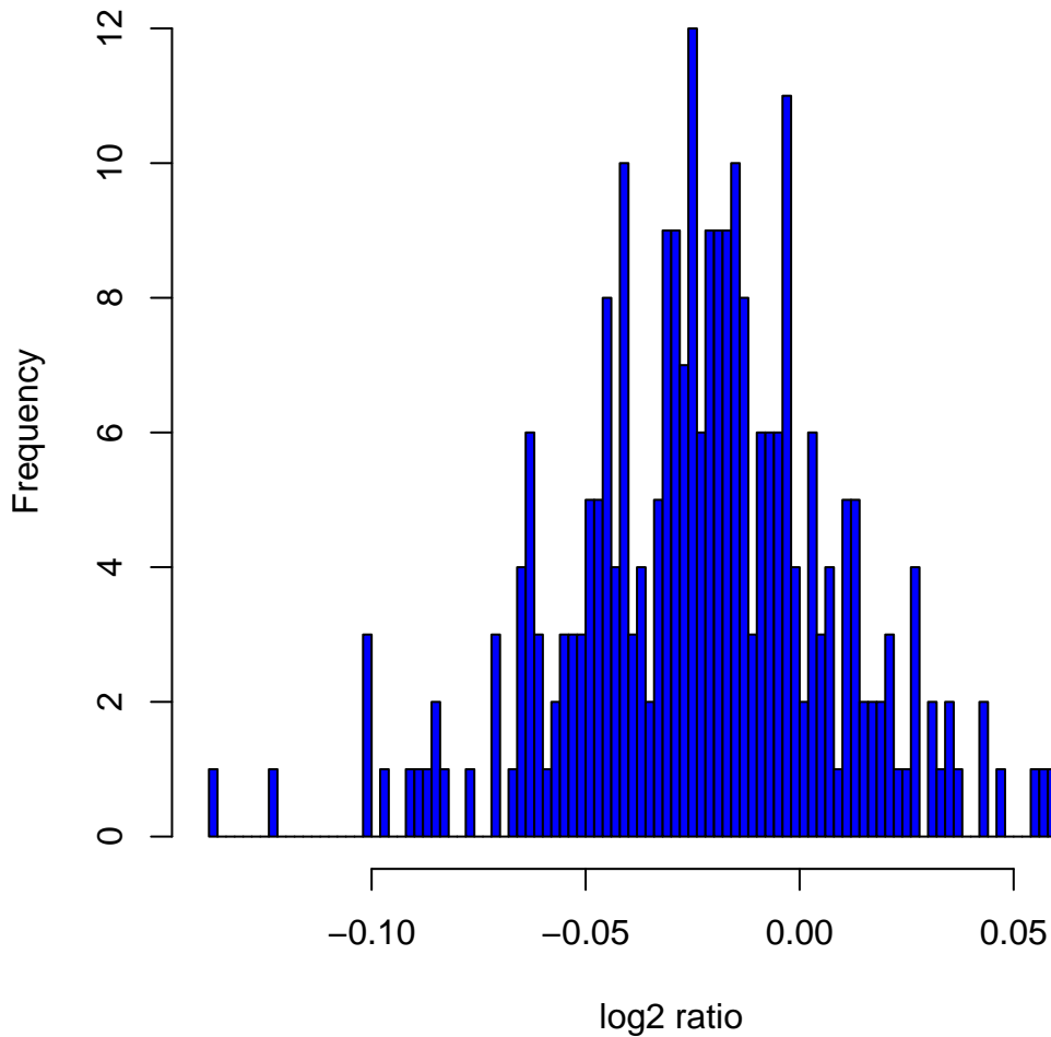
Histogram of log 2 ratios in 270 HapMap samples at clone Chr7tp-8H6
