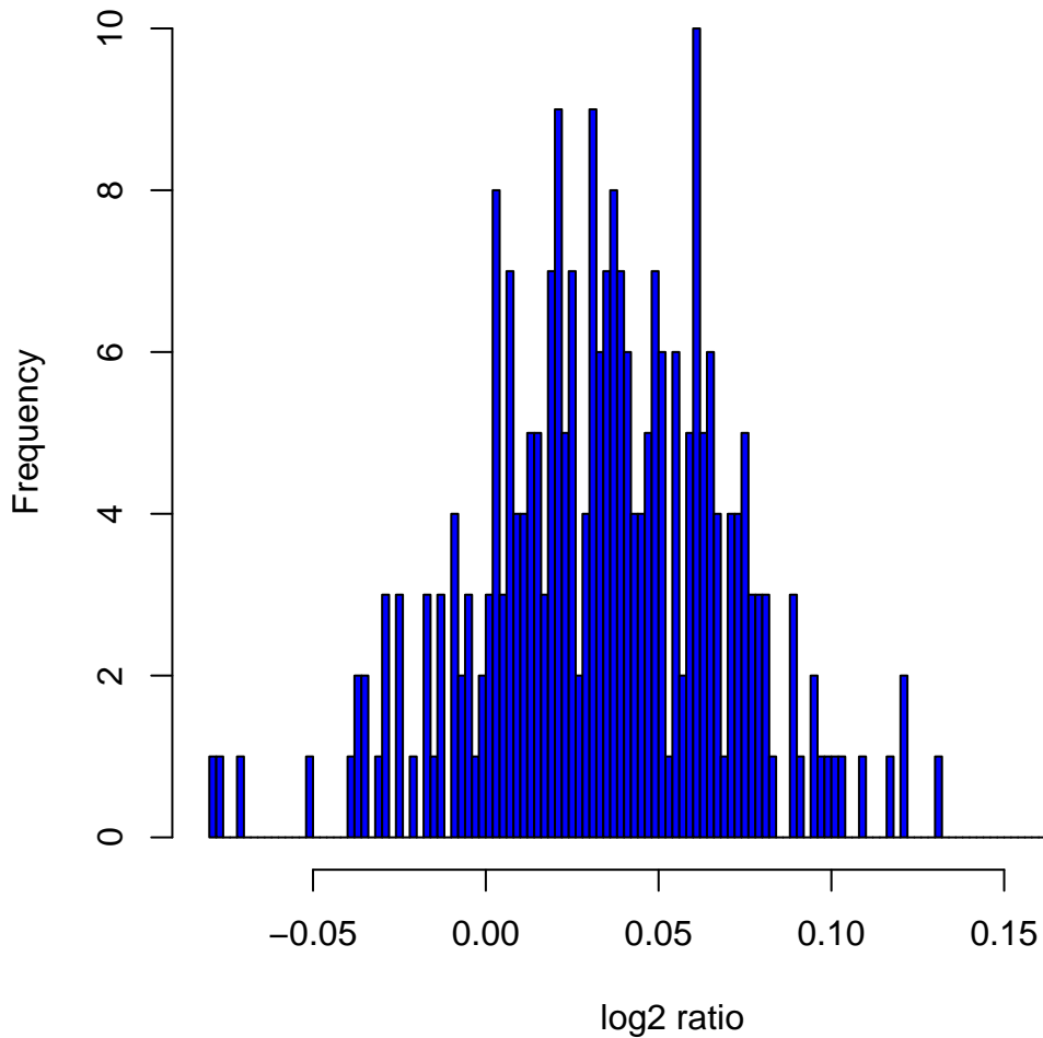
Histogram of log 2 ratios in 270 HapMap samples at clone Chr7tp-9A5
