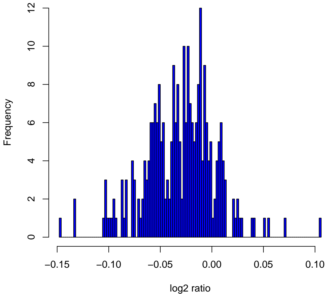
Histogram of \log_2 ratios in 270 HapMap samples at clone Chr7tp-9A9
