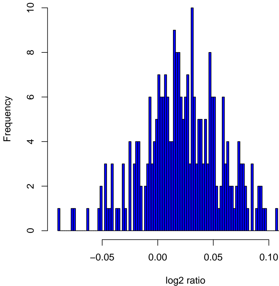
Histogram of log2ratios in 270 HapMap samples at clone Chr7tp-9F8
