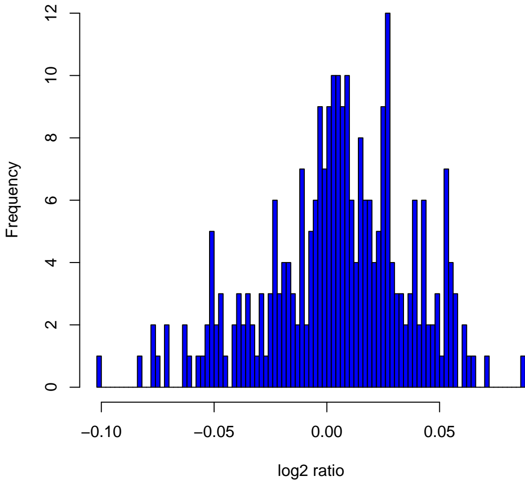
Histogram of log2ratios in 270 HapMap samples at clone Chr8tp-10A10
