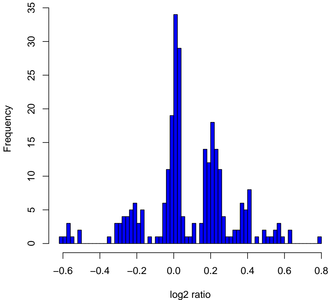
Histogram of log 2 ratios in 270 HapMap samples at clone Chr8tp-10C3
