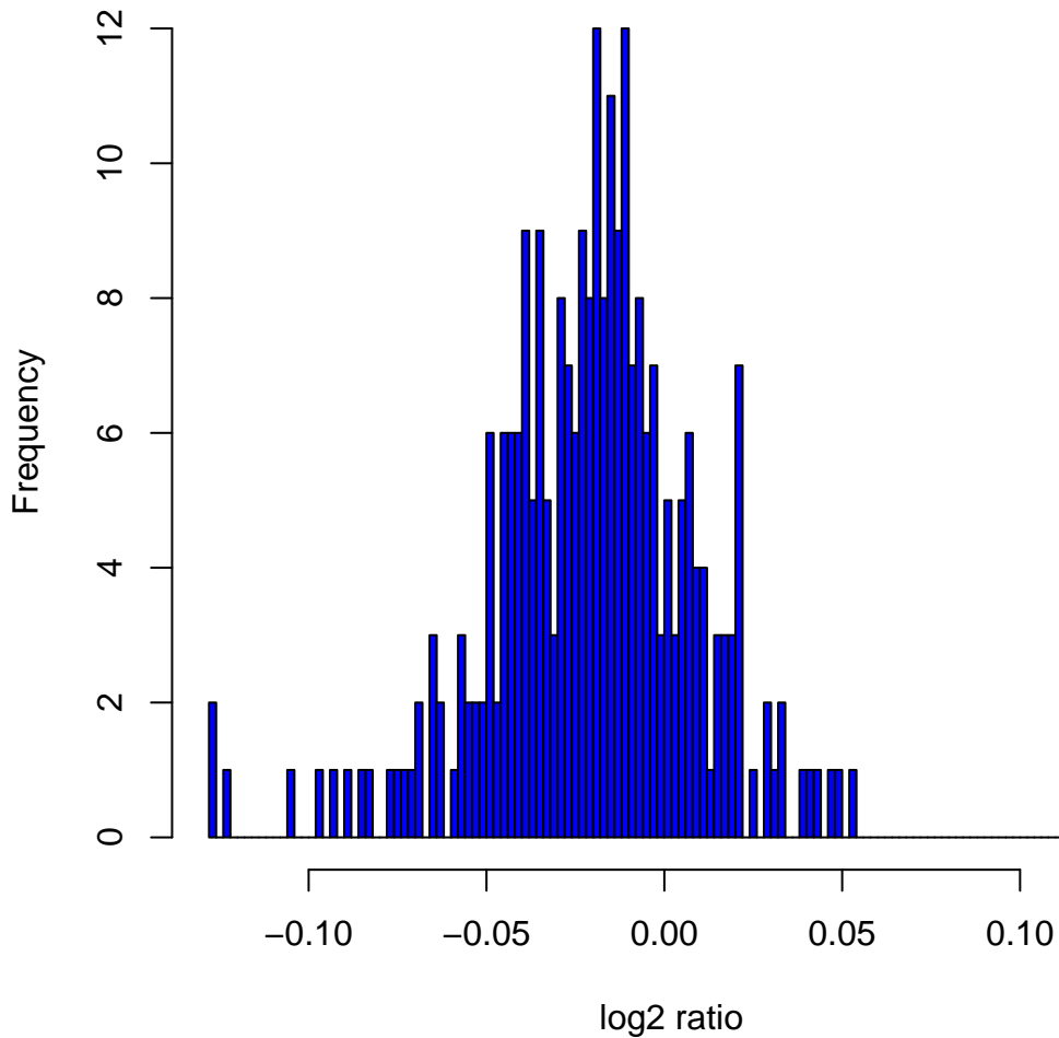
Histogram of log 2 ratios in 270 HapMap samples at clone Chr8tp-10C9
