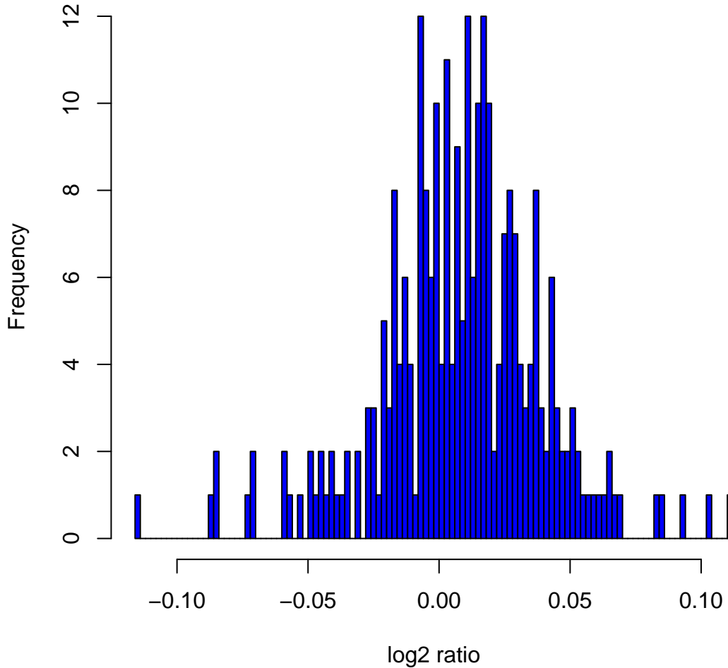
Histogram of log 2 ratios in 270 HapMap samples at clone Chr8tp-10D2
