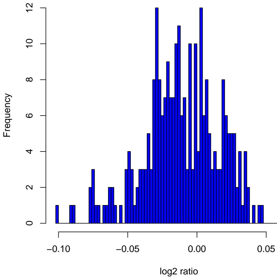
Histogram of log 2 ratios in 270 HapMap samples at clone Chr8tp-10D5
