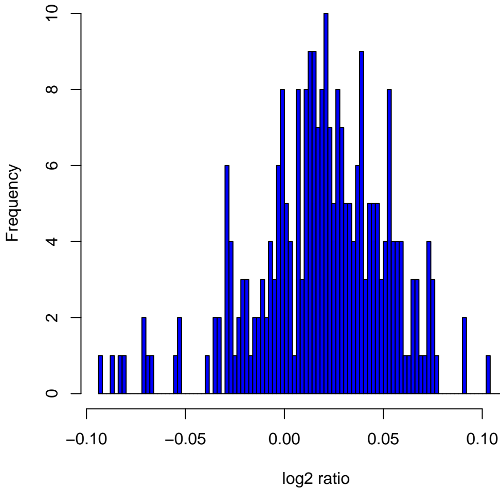
Histogram of \log_2 ratios in 270 HapMap samples at clone Chr8tp-10G3
