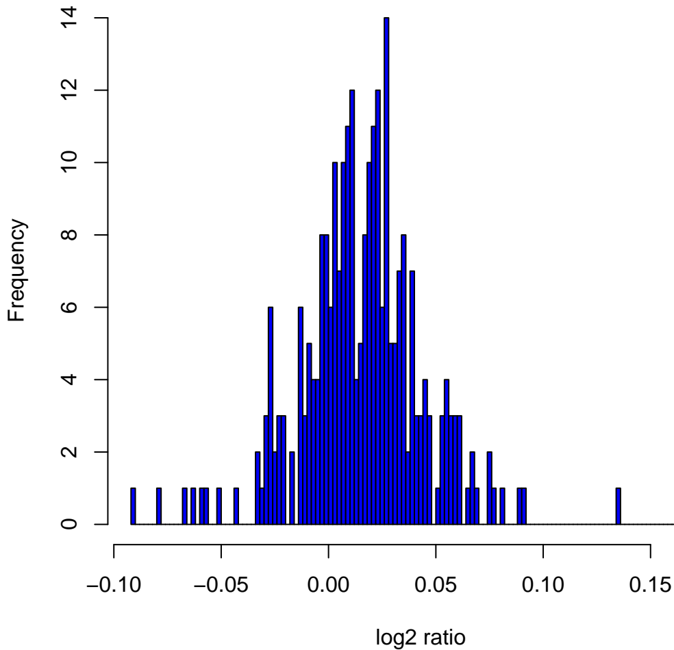
Histogram of log 2 ratios in 270 HapMap samples at clone Chr8tp-11B2
