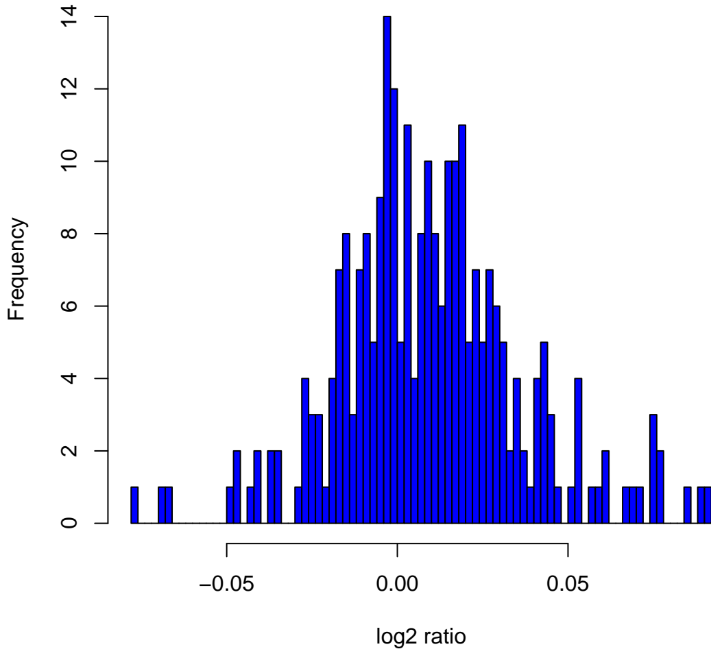
Histogram of log2ratios in 270 HapMap samples at clone Chr8tp-11D1
