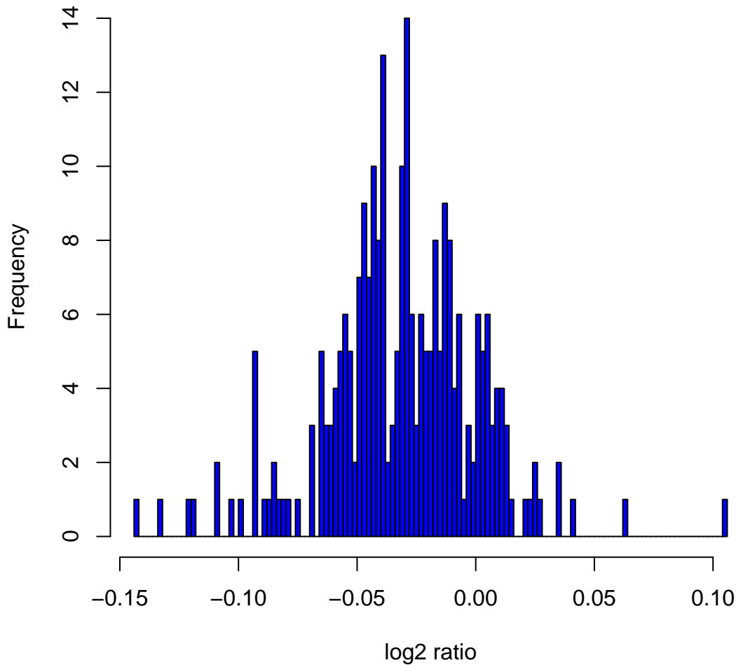
Histogram of log 2 ratios in 270 HapMap samples at clone Chr8tp-11D9
