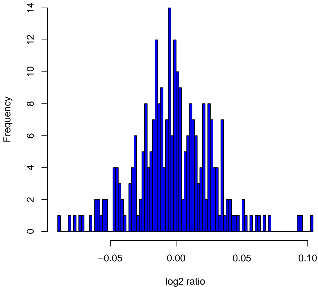
Histogram of \log_2 ratios in 270 HapMap samples at clone Chr8tp-11G2
