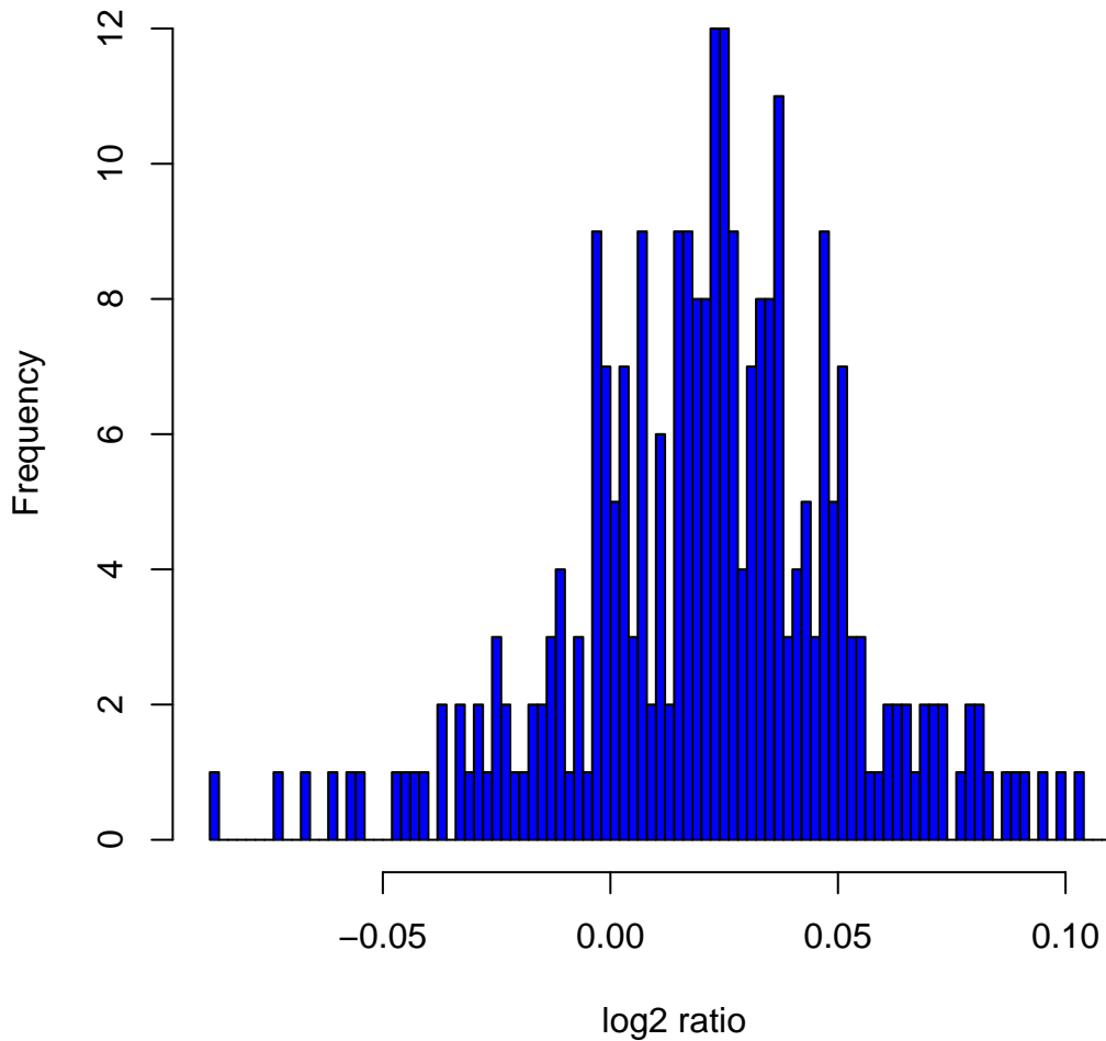
Histogram of log 2 ratios in 270 HapMap samples at clone Chr8tp-16E2
