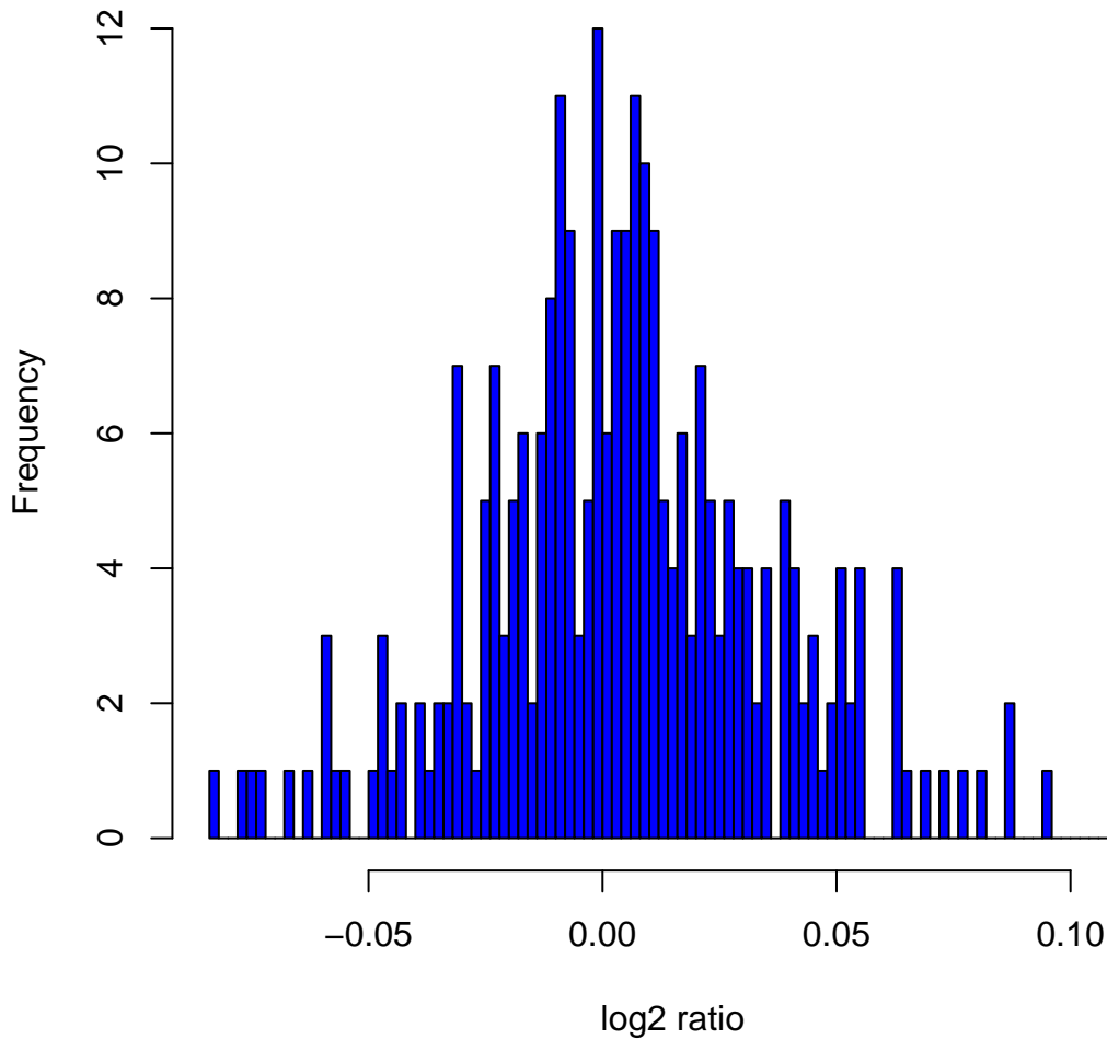
Histogram of log 2 ratios in 270 HapMap samples at clone Chr8tp-16E4
