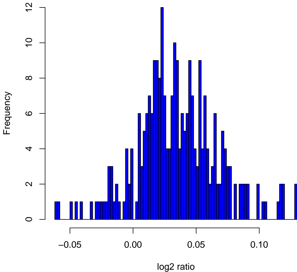
Histogram of \log_2 ratios in 270 HapMap samples at clone Chr8tp-16G1
