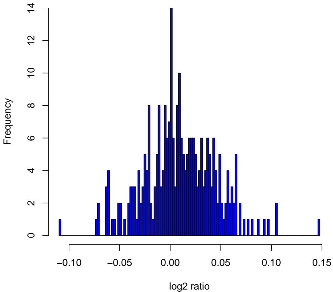
Histogram of log 2 ratios in 270 HapMap samples at clone Chr8tp-17G6
