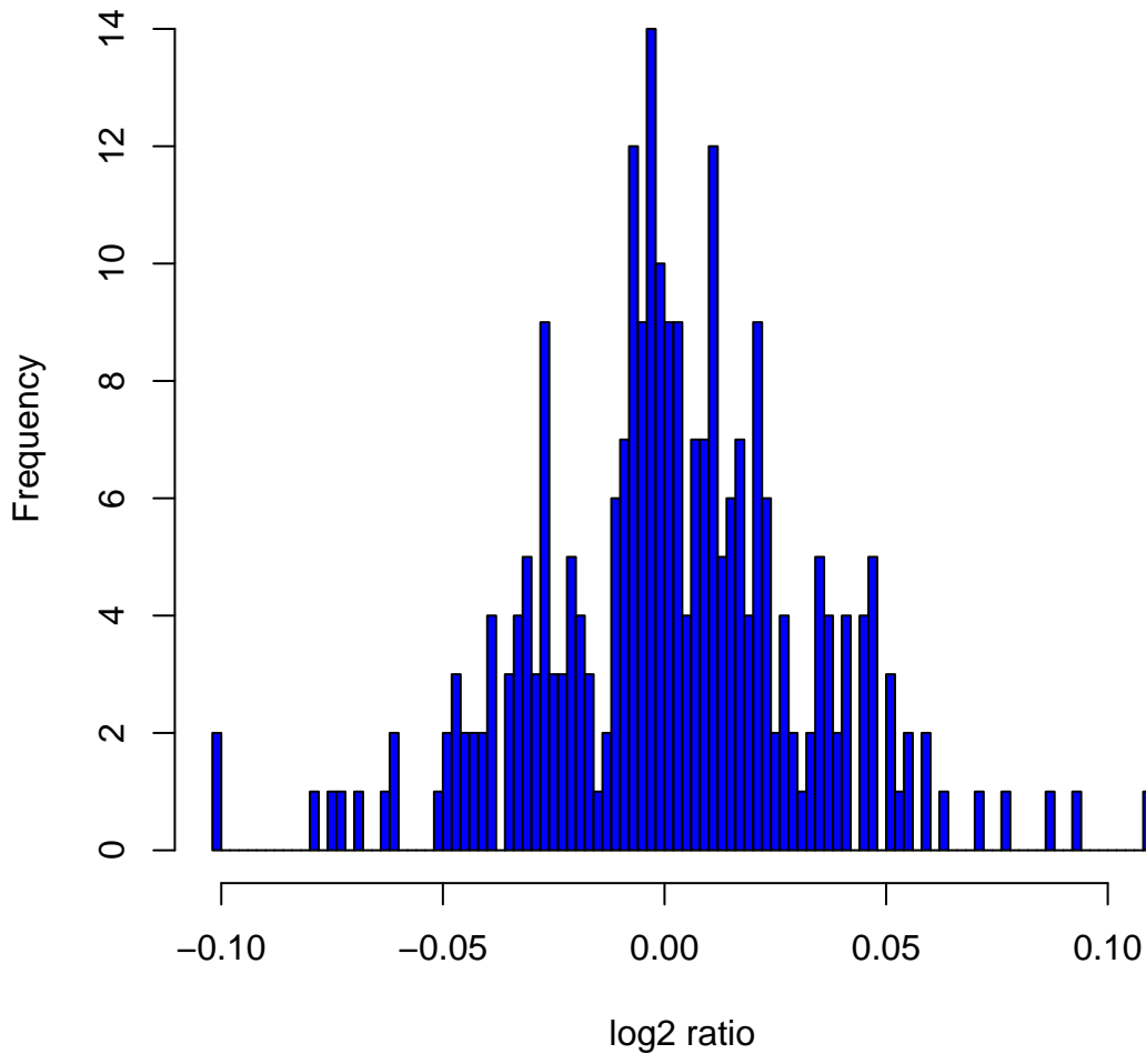
Histogram of log 2 ratios in 270 HapMap samples at clone Chr8tp-17H7
