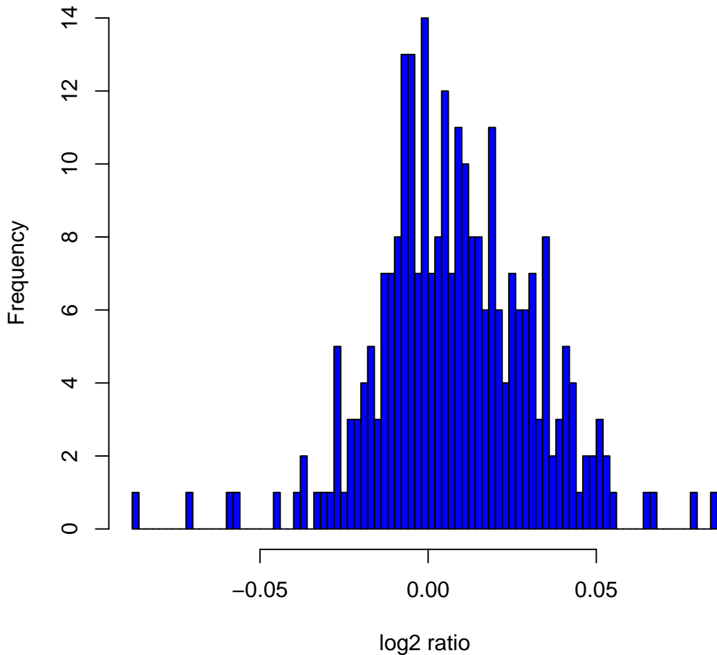
Histogram of log2ratios in 270 HapMap samples at clone Chr8tp-18A1
