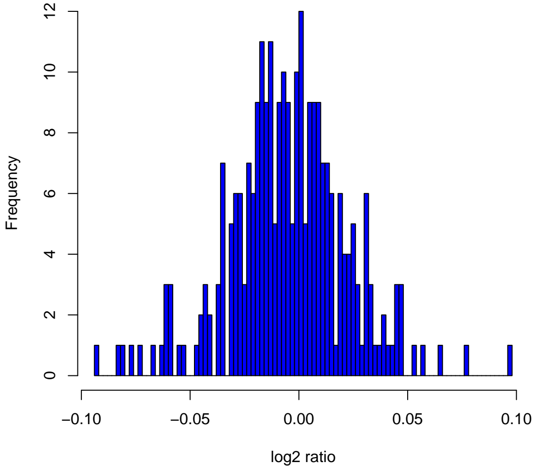
Histogram of log2ratios in 270 HapMap samples at clone Chr8tp-18B11
