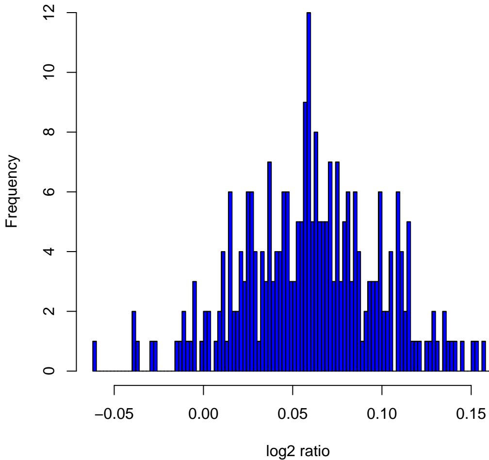
Histogram of log2ratios in 270 HapMap samples at clone Chr8tp-18C12
