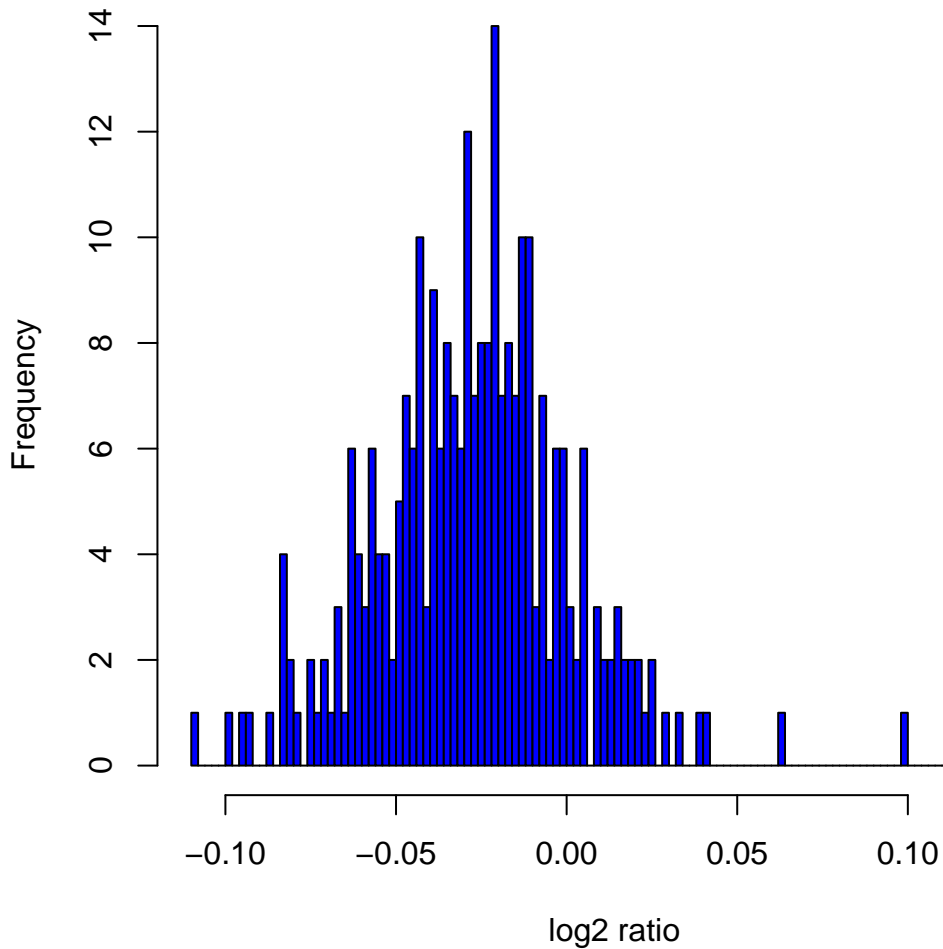
Histogram of log 2 ratios in 270 HapMap samples at clone Chr8tp-18C7
