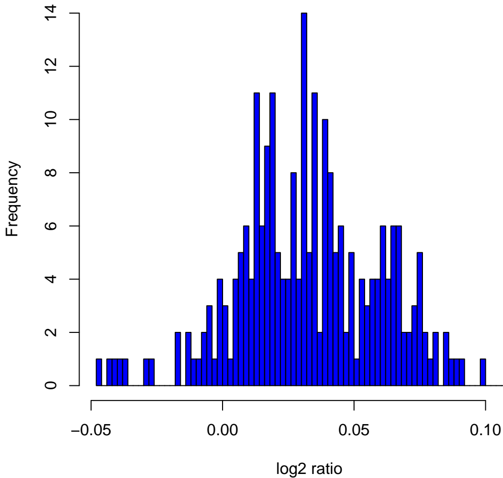
Histogram of log2ratios in 270 HapMap samples at clone Chr8tp-18D12
