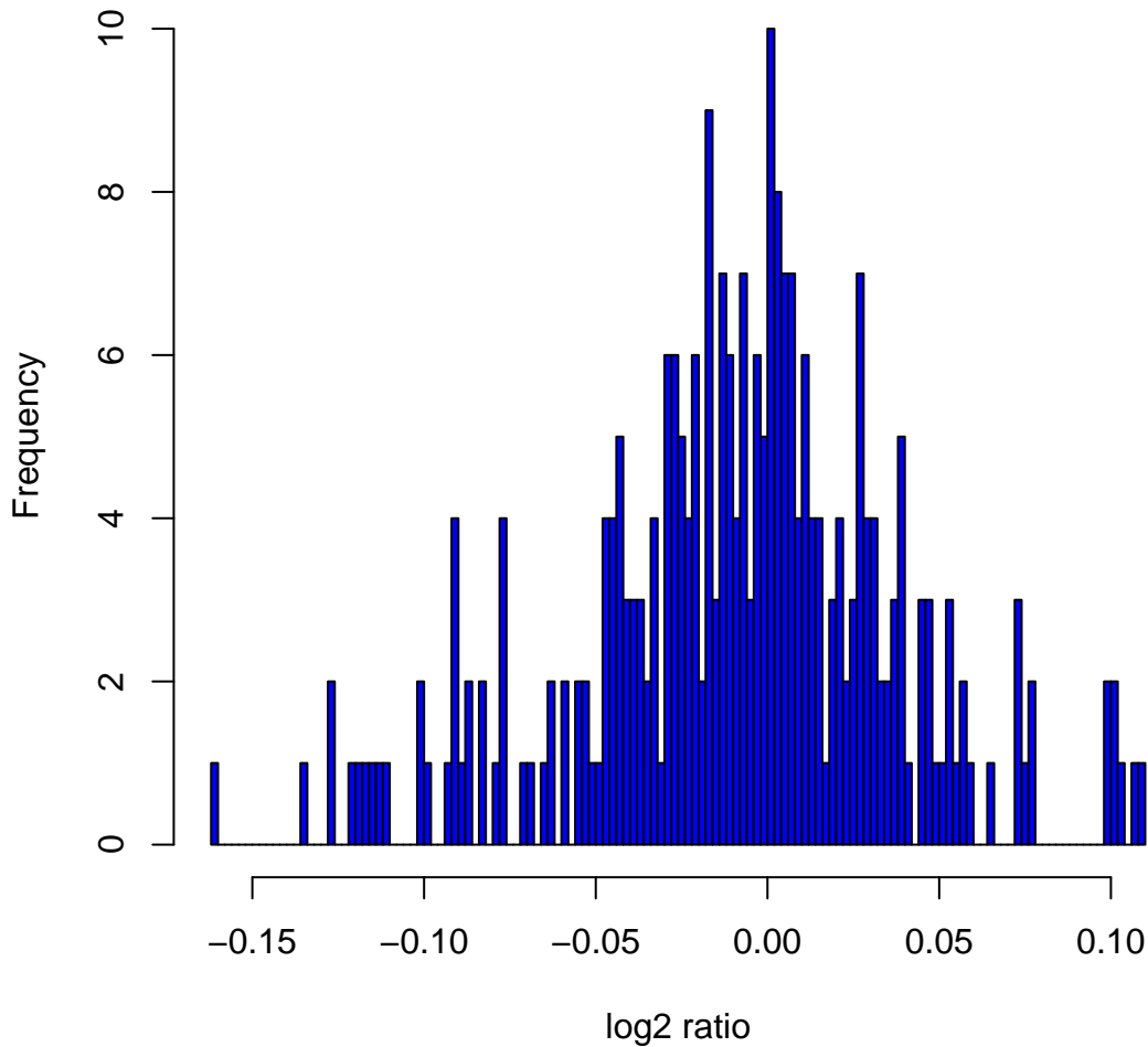
Histogram of log 2 ratios in 270 HapMap samples at clone Chr8tp-18G4
