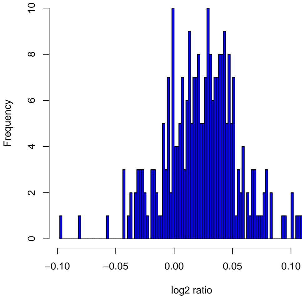
Histogram of log 2 ratios in 270 HapMap samples at clone Chr8tp-19C3
