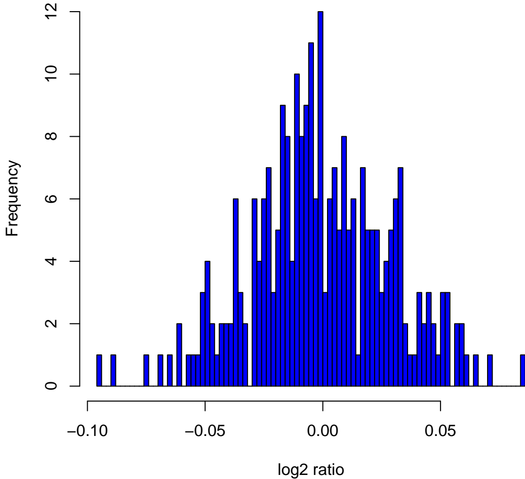
Histogram of log2ratios in 270 HapMap samples at clone Chr8tp-19D11
