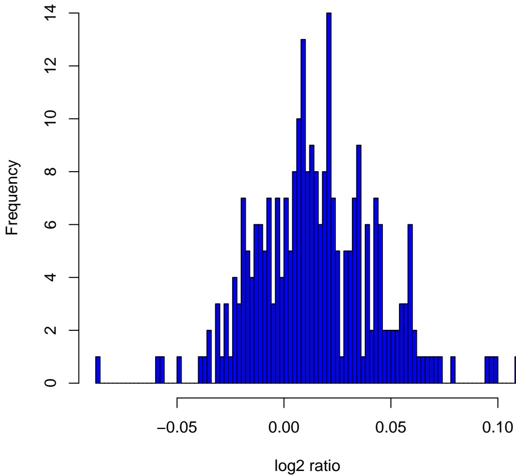
Histogram of log 2 ratios in 270 HapMap samples at clone Chr8tp-19D2
