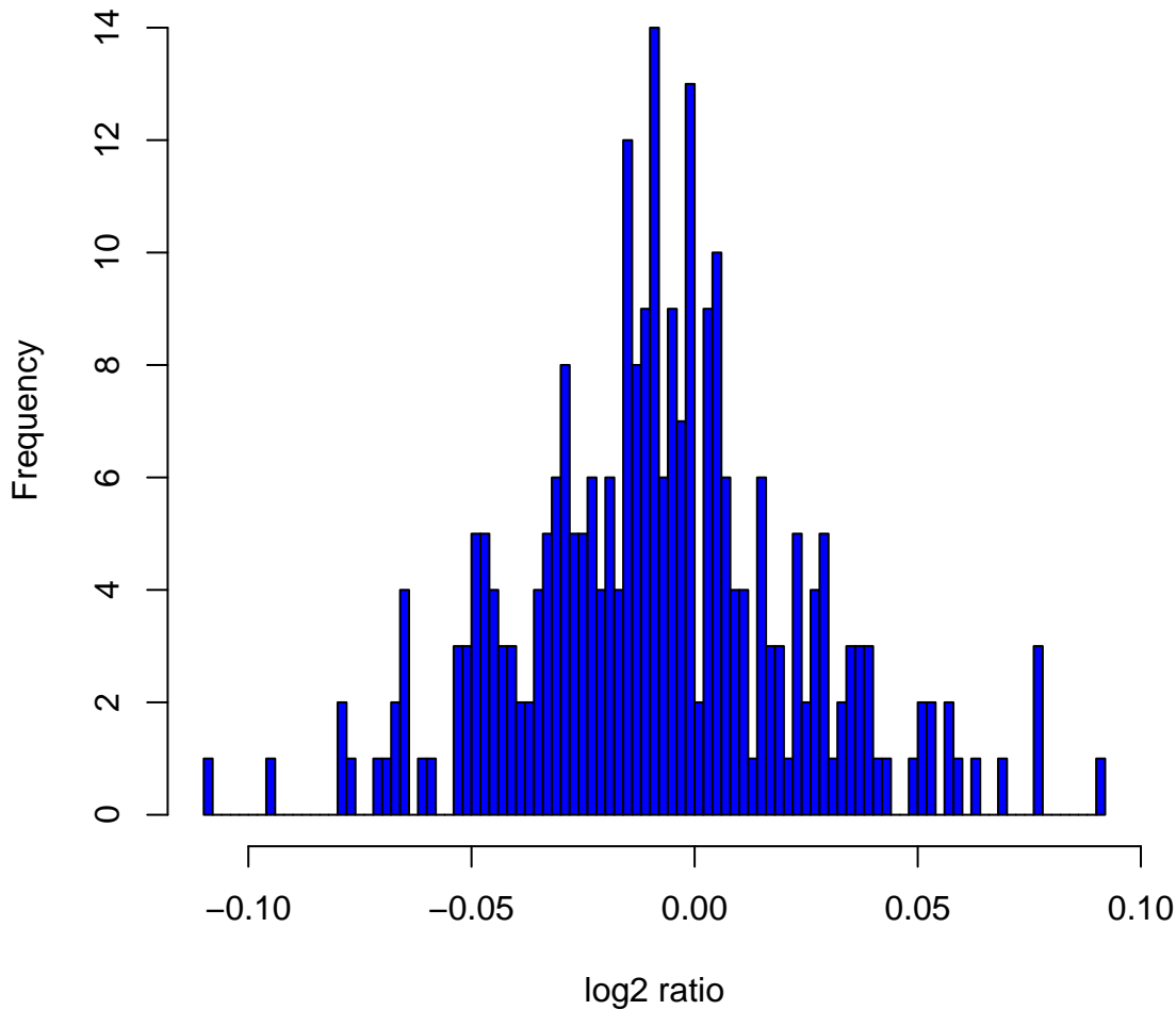
Histogram of log 2 ratios in 270 HapMap samples at clone Chr8tp-19D9
