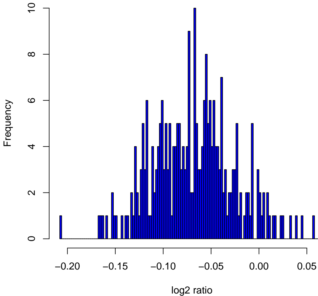
Histogram of \log_2 ratios in 270 HapMap samples at clone Chr8tp-19E4
