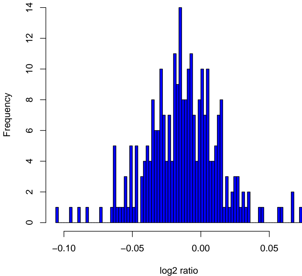
Histogram of log 2 ratios in 270 HapMap samples at clone Chr8tp-1B6
