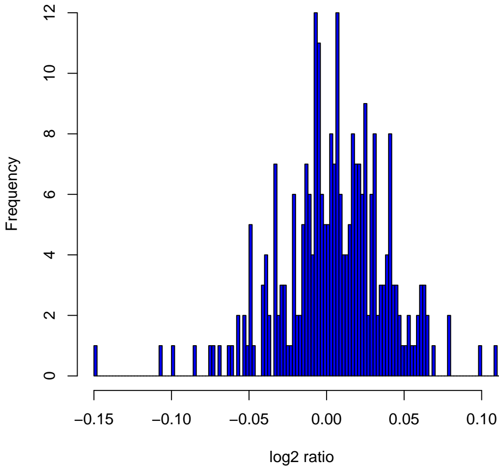
Histogram of log 2 ratios in 270 HapMap samples at clone Chr8tp-1C8
