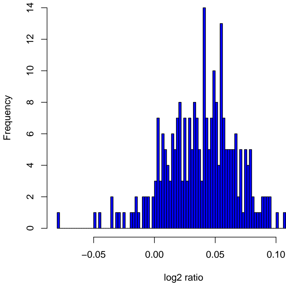
Histogram of log 2 ratios in 270 HapMap samples at clone Chr8tp-1D10
