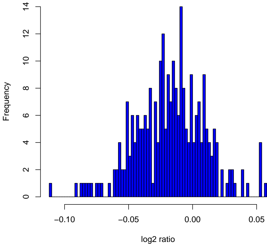
Histogram of log 2 ratios in 270 HapMap samples at clone Chr8tp-1D5
