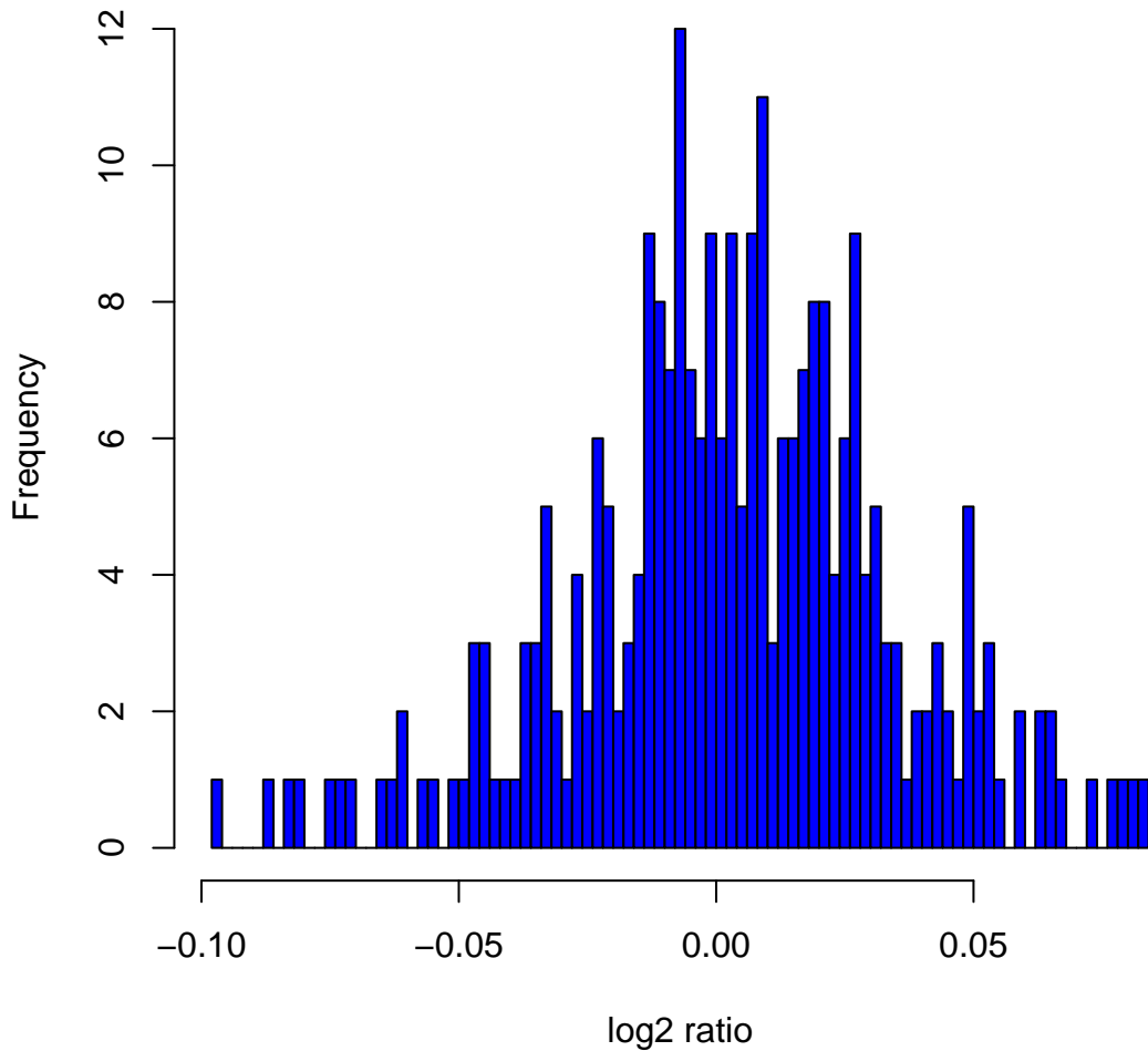
Histogram of log2ratios in 270 HapMap samples at clone Chr8tp-1E3
