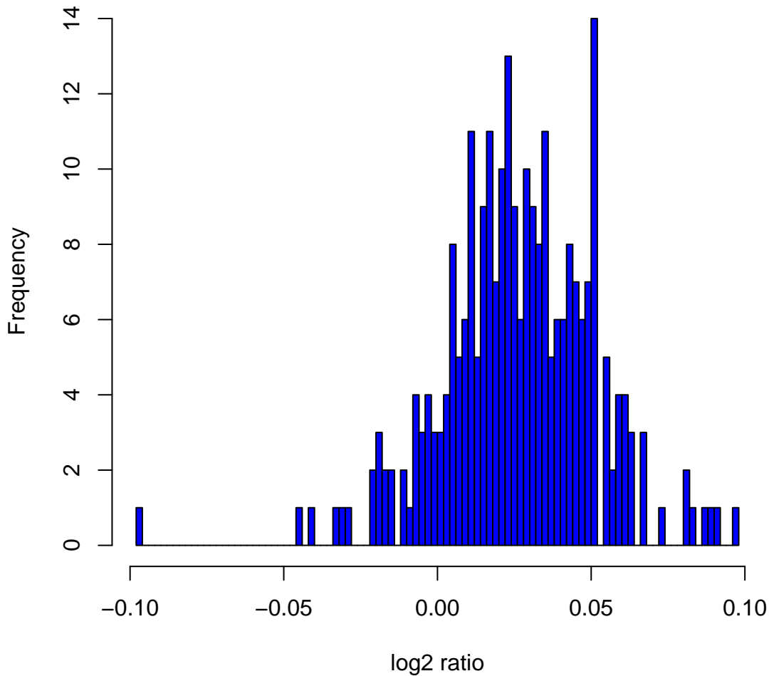
Histogram of log 2 ratios in 270 HapMap samples at clone Chr8tp-1E8
