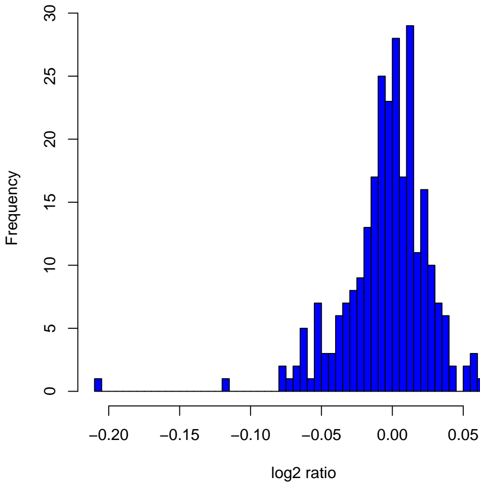
Histogram of log 2 ratios in 270 HapMap samples at clone Chr8tp-1F3
