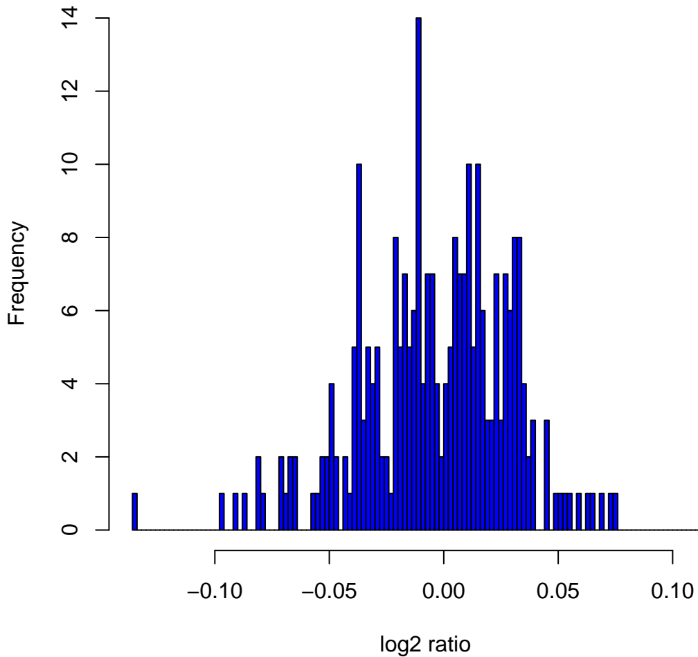
Histogram of log 2 ratios in 270 HapMap samples at clone Chr8tp-1G2
