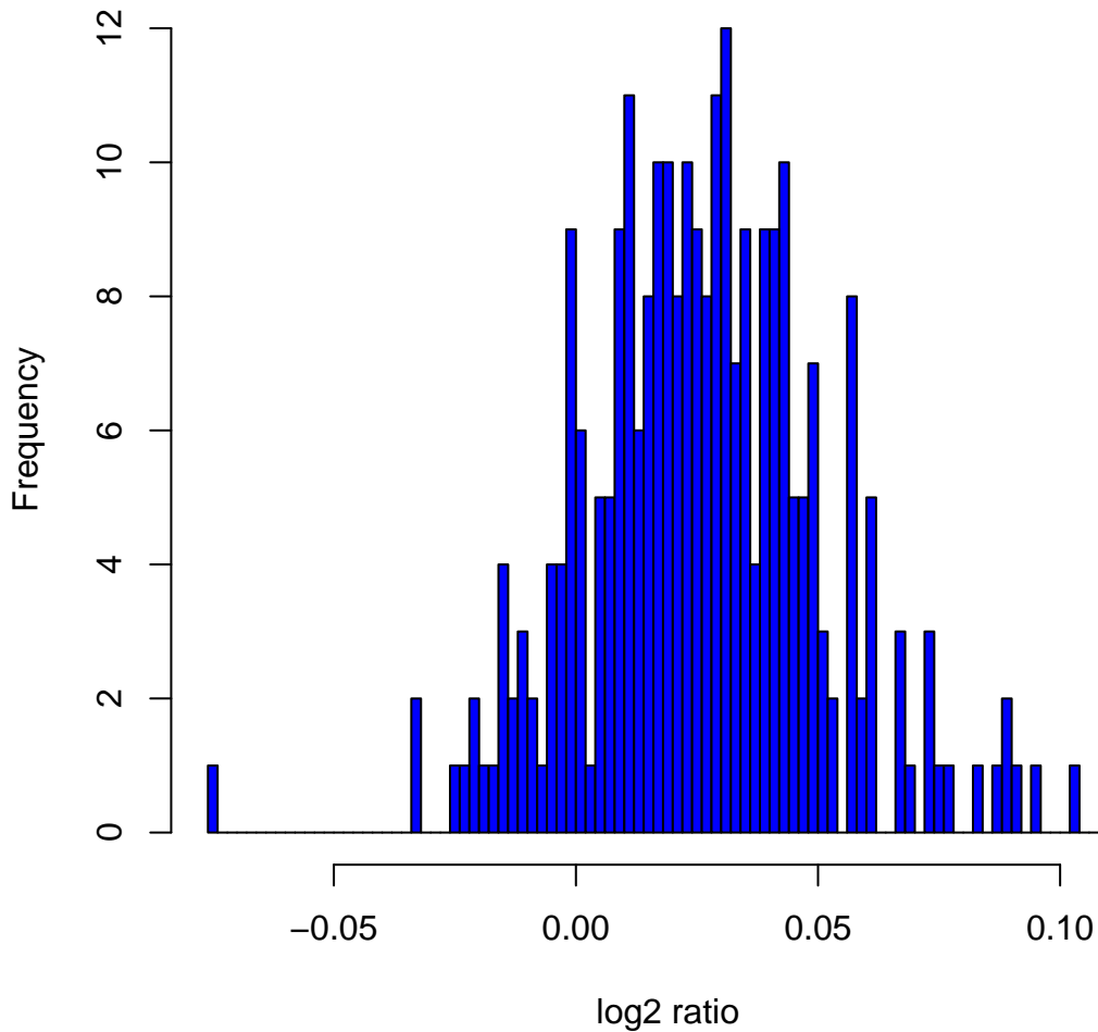
Histogram of log 2 ratios in 270 HapMap samples at clone Chr8tp-1G3
