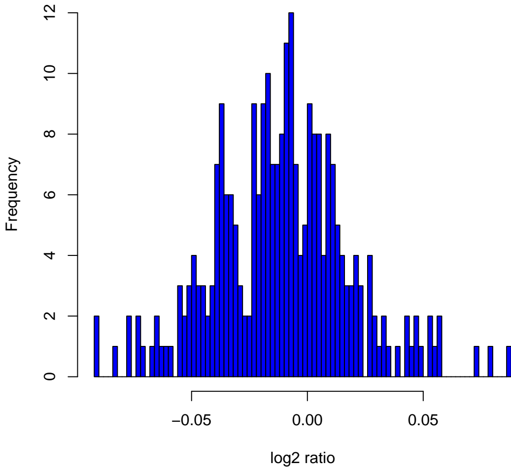
Histogram of log2ratios in 270 HapMap samples at clone Chr8tp-20A12
